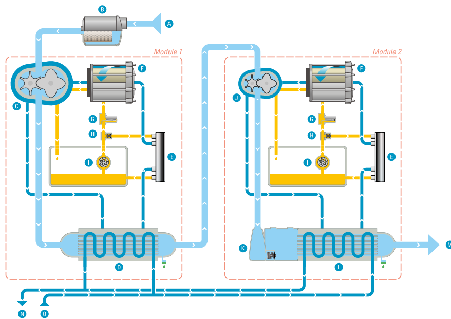
ZR 90 - 160 VSD*
